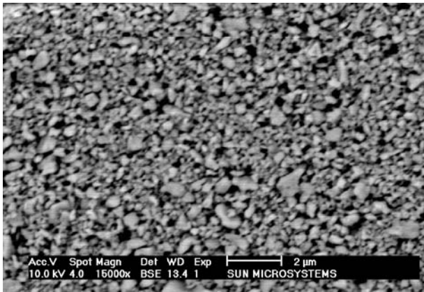
Figure 2 Plan view of scanning electron micrograph of an alumina deposit produced by EPD.
