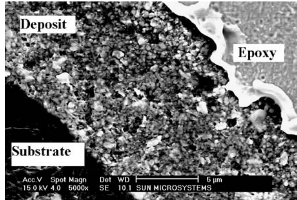
Figure 4 Cross-section of deposit after 15 s of electrophoretic deposition.
